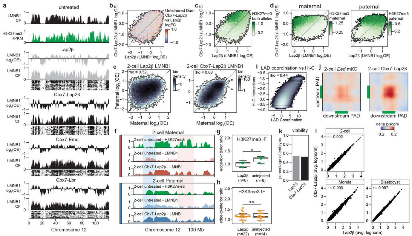
Extended Data Fig. 6 | Effect of H3K27me3-tethering to the NL nuclear lamina. a , Single-cell heatmaps of binarized LMNB1 profiles of Lap2 \beta , Cbx7-Lap2 \beta , Cbx7-Emd , Cbx7-Lbr 2-cell embryos with corresponding CF and log 2 (OE) values along chromosome 12. On top, 2-cell LMNB1 CF and H3K27me3 (ref. 13) of untreated embryos are shown. b , Comparison of LMNB1 values in 100-kb bins for the Cbx7-Lap2 \beta and the Lap2 \beta conditions. The color indicates the average log 2 (FC) of untethered Dam between Cbx7-Lap2 \beta and Lap2 \beta embryos. c-d , Comparison of LMNB1 values in the Cbx7-Lap2 \beta and Lap2 \beta -injected hybrid embryos for both alleles ( c ) or maternal and paternal alleles separately ( d ). The color scale indicates the average allele-specific H3K27me3 values of 2-cell WT embryos. e , Comparison of paternal and maternal LMNB1 CF in Lap2 \beta (left, \rho = 0.32 , p < 1e-100 , n = 21,710 bins) and Cbx7-Lap2 \beta conditions (right, \rho = 0.68 , p < 1e-100 , n = 21,710 bins). Correlations were computed using Spearman's rank-order correlation. f , Example genomic region with maternal (top) and paternal (bottom) LMNB1 CF for Cbx7-Lap2 \beta and Lap2 \beta conditions and 2-cell WT H3K27me3. Dashed boxes highlight examples of allelic LAD asymmetry in the Cbx7-Lap2 \beta condition: paternal-specific LADs in blue and maternal-specific LADs in red. g-h , Quantification of the radial (1 \mu m) enrichment of H3K27me3 ( g ) and H3K9me3 ( h ) relative to the rest of the nucleus. Significance was computed using Welch's two-sided t-test (H3K27me3, p = 0.024 ; H3K9me3, p = 0.96 ). H3K27me3: Lap2 \beta , n = 6 ; uninjected, n = 6 . H3K9me3: Lap2 \beta , n = 22 ; uninjected, n = 14 . Data is from one biological replicate. Boxplots indicate median values (white line), inter-quartile range (IQR, black box) and the range within 1.5 times the IQR (whiskers). i , Correlation between LAD coordination metric and Hi-C interaction values up to 50 Mb distance ( \rho = 0.44 , p < 1e-100 , n = 5,311,617 100-kb bin pairs). j , Average LAD coordination between PAD pairs up to 20 Mb distance. k , Fraction of embryos reaching the blastocyst stage (E3.5) in Cbx7-Lap2 \beta and Lap2 \beta conditions ( Cbx7-Lap2 \beta , n = 67 ; Lap2 \beta , n = 65 ). Data is from one biological replicate. l , Gene expression comparison between Cbx7-Lap2 \beta and Lap2 \beta embryos at 2-cell, morula and blastocyst stages. No significant differentially expressed genes were detected. Pearson's correlation was computed (2-cell, p < 2.2e-16 , n = 14,862 genes; morula, p < 2.2e-16 , n = 15,259 genes; blastocyst, p < 2.2e-16 , n = 15,259 genes). Correlations in ( e ) and ( g ) were computed using Spearman's rank-order correlation.
